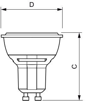
LED VLE D 4.3-50W GU10 840 40D
