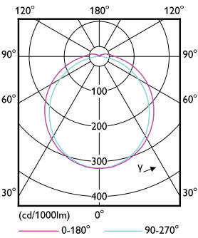
Light Distribution Diagram - LED PLC 8.9W 840 2P G24d-3
