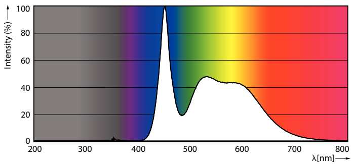
Spectral Power Distribution Colour - EcoHome LEDBulb 12W E27 6500KLV 1PF/20
