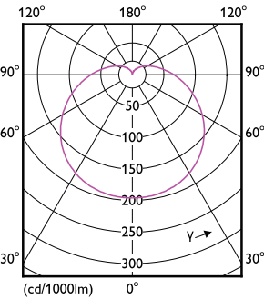
Light Distribution Diagram - EcoHome LEDBulb 12W E27 3000KLV 1PF/20
