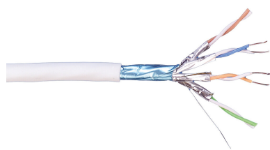
CS54Z3 Category 7 F/FTP Cable, low smoke zero halogen, white jacket, 4 pair count, 1640 ft (500 m) length, reel
